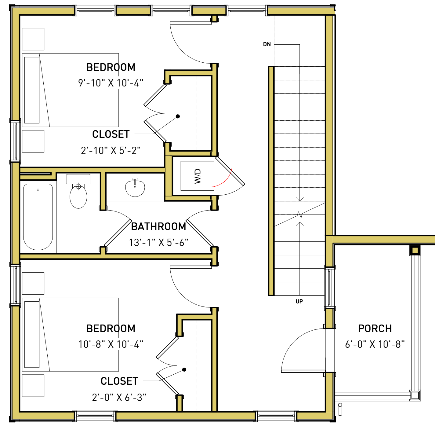
2 2ND FLOOR SD-2.1 1/4" = 1'-0"
