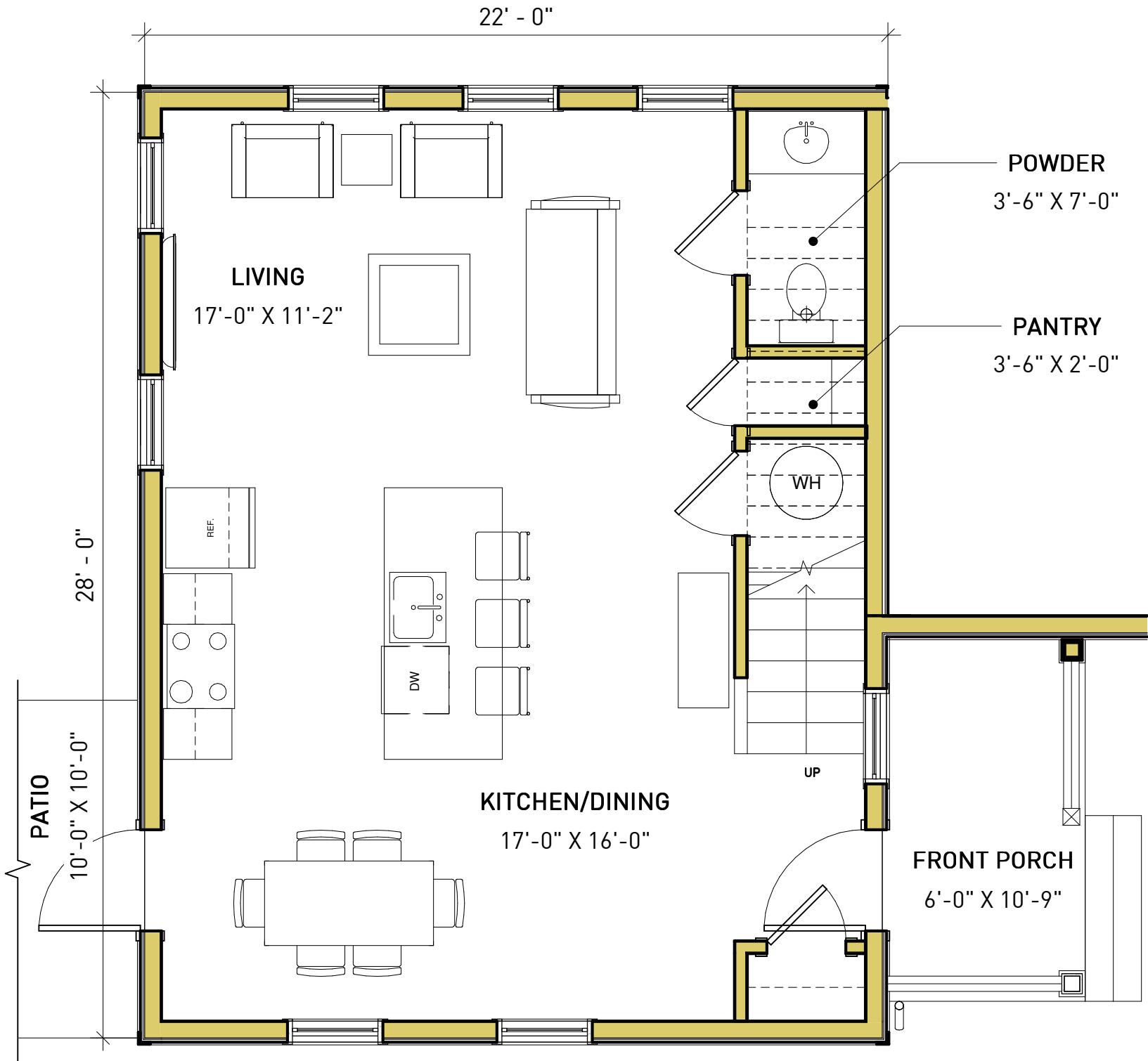
1 1ST FLOOR SD-2.1 1/4" = 1'-0"
