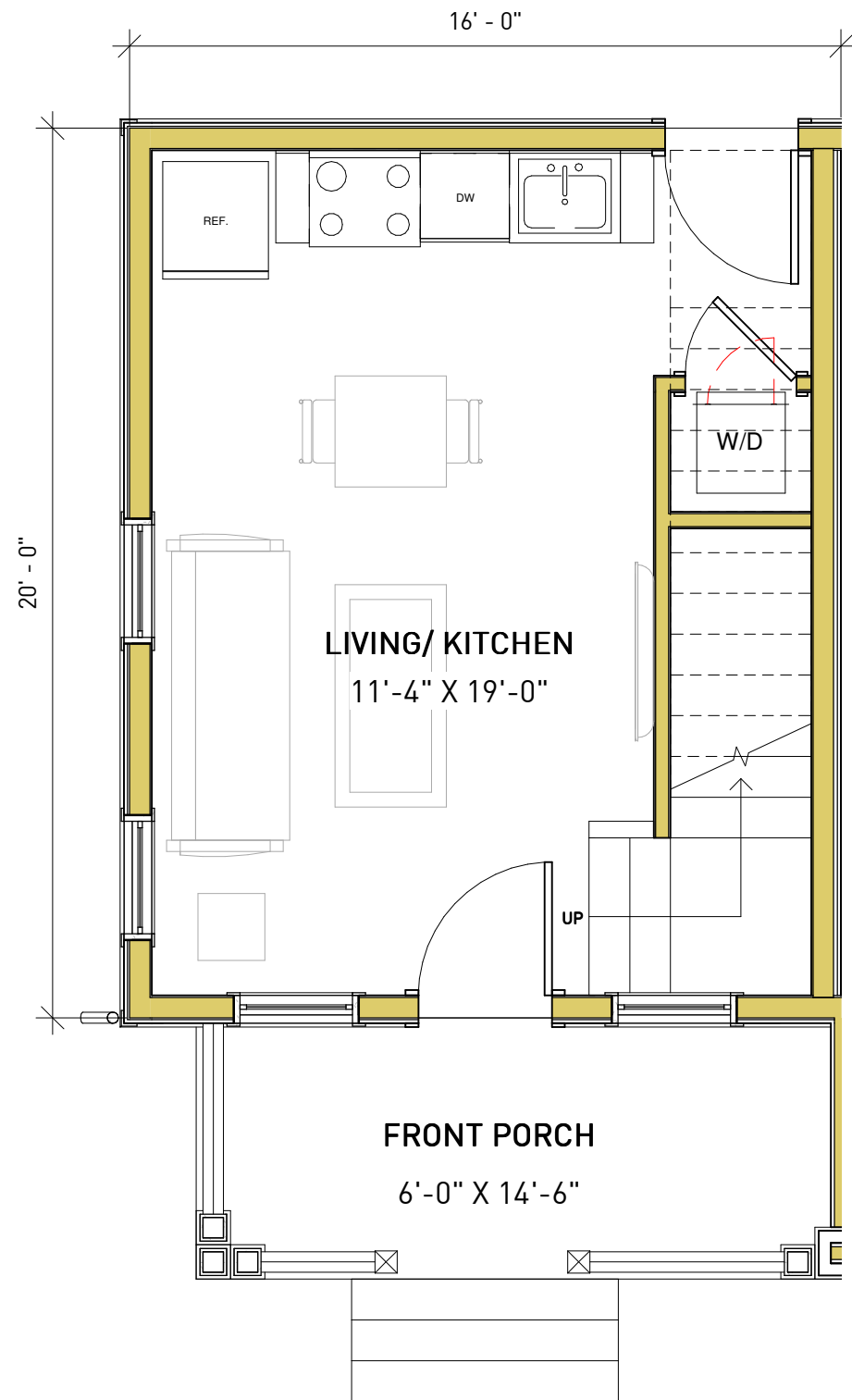
1 1ST FLOOR PLAN SD-2.1 1/4" = 1'-0"
