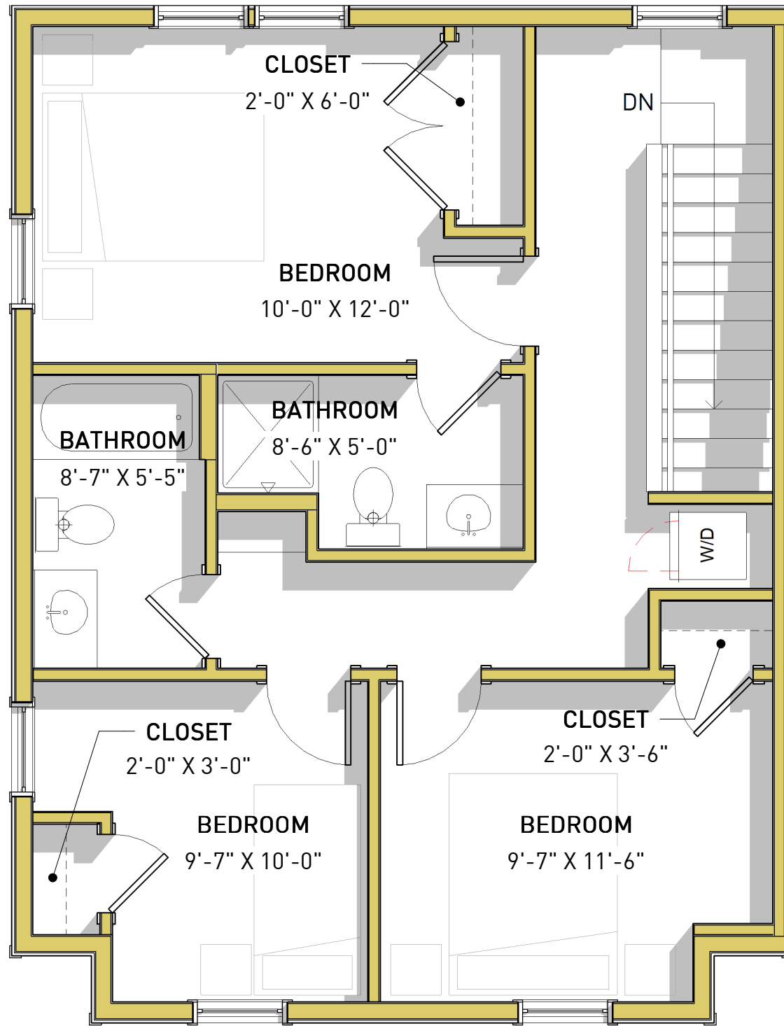
2 2ND FLOOR PLAN MK-2.1 1/4" = 1'-0"
