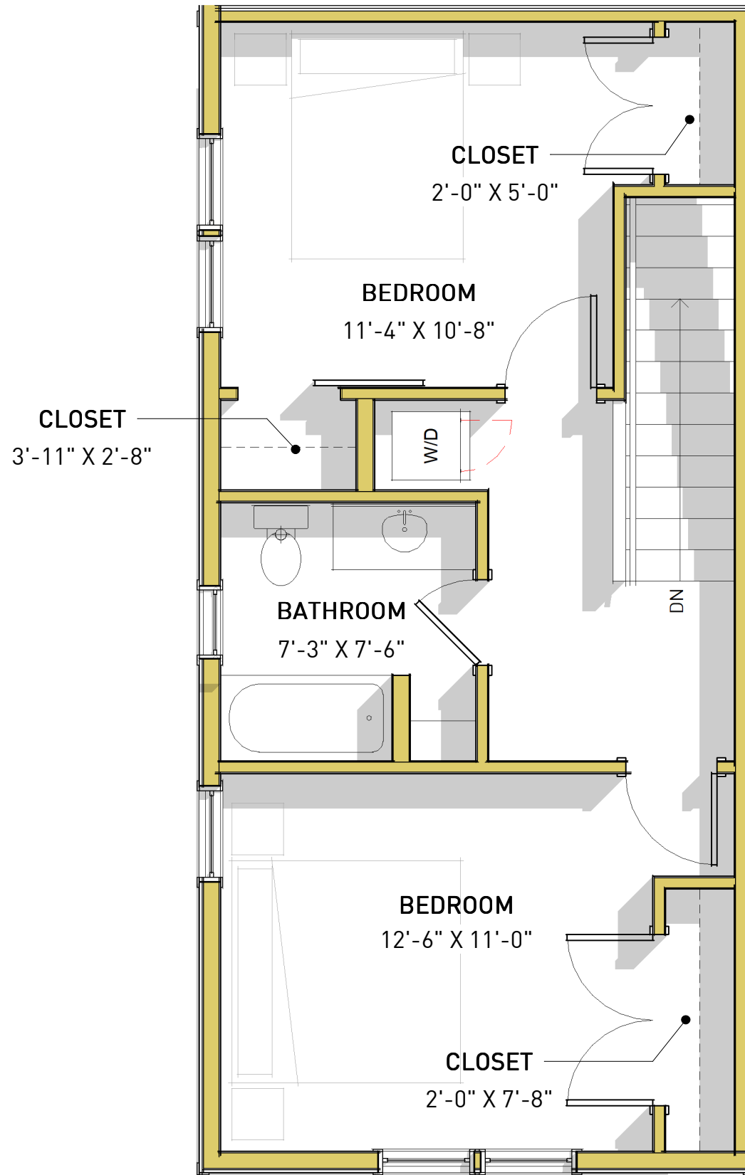
2 2ND FLOOR PLAN MK-2.4 1/4" = 1'-0"
